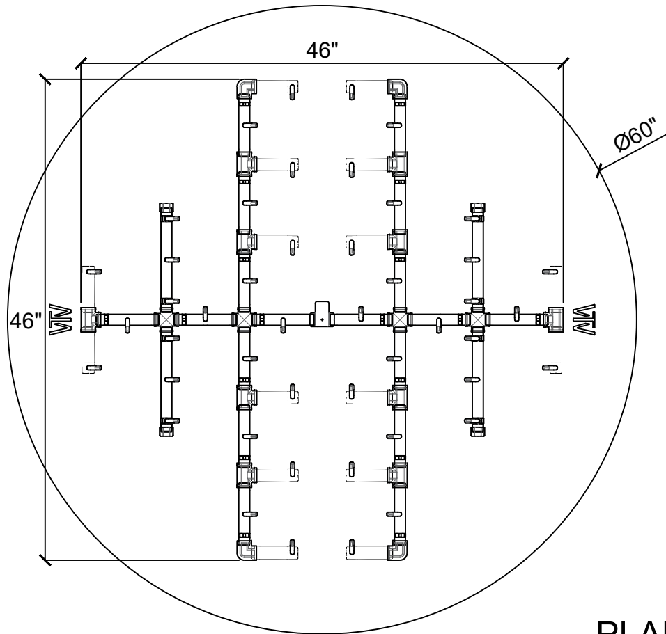
PLAN VIEW
