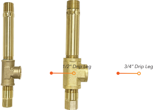
Photo 6: Drip Legs
