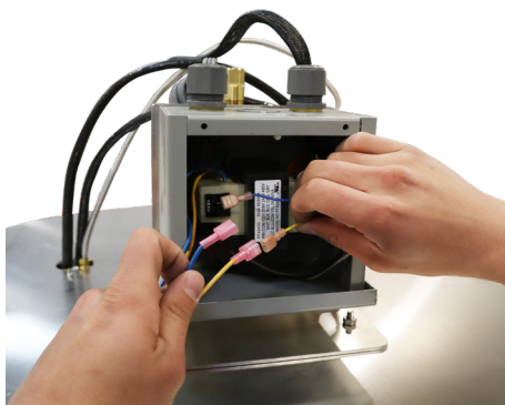
Photo 17: Connecting the Valve to the Transformer
