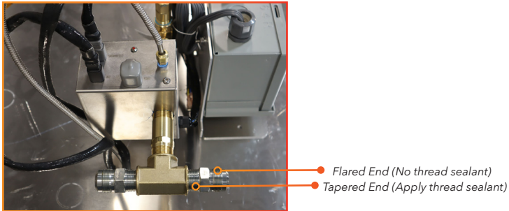
Photo 26: Connecting the Flared Fittings and 3/4" Tee to the 3" Nipple
