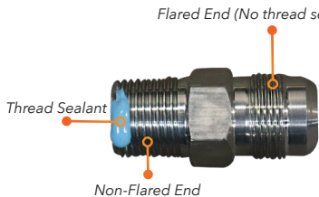
Photo 19: Flared Fitting with Thread Sealant
