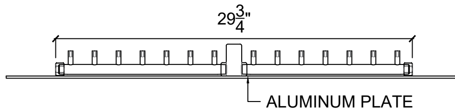
ELEVATION VIEW
