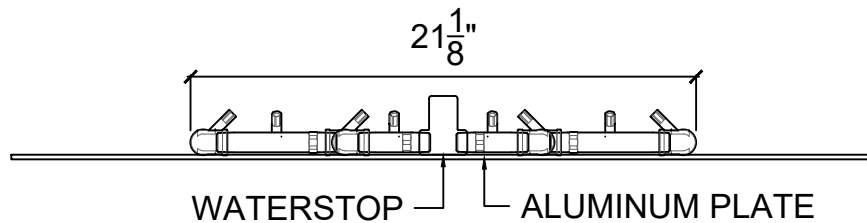
ELEVATION VIEW
