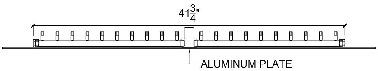
ELEVATION VIEW
