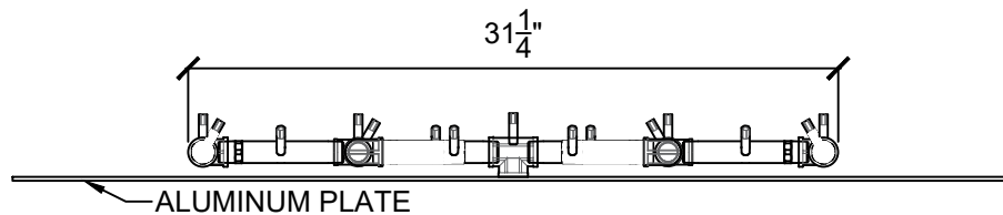
ELEVATION VIEW
