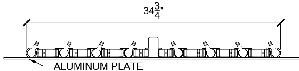
ELEVATION VIEW
